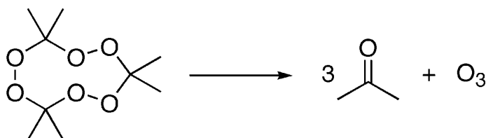
Triacetone-triperoxide (TATP)
